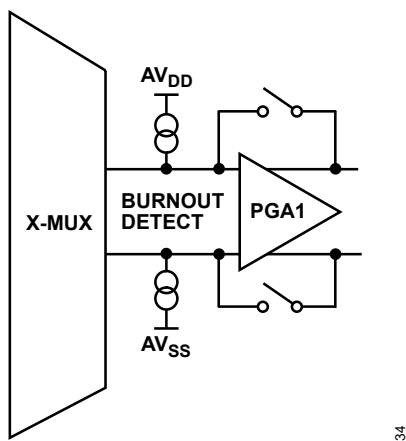
Figure 124. Burnout Currents
