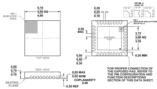
Figure 129. 32-Lead Lead Frame Chip Scale Package [LFCSP] 5 mm x 5 mm Body and 0.75 mm Package Height (CP-32-12) Dimensions shown in millimeters
