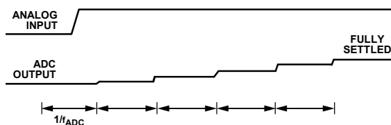
Figure 83. Asynchronous Step Change in the Analog Input
