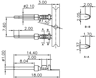
Male terminal
