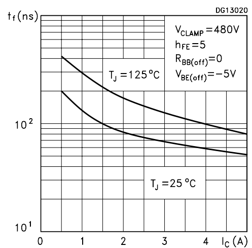
Inductive Load Fall Time
