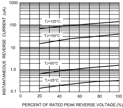
FIG.3-TYPICAL REVERSE CHARACTERISTICS
