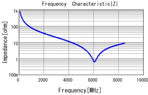
■ GCM1555C1H2R0BA16 |Z| DCOV, 25degC
