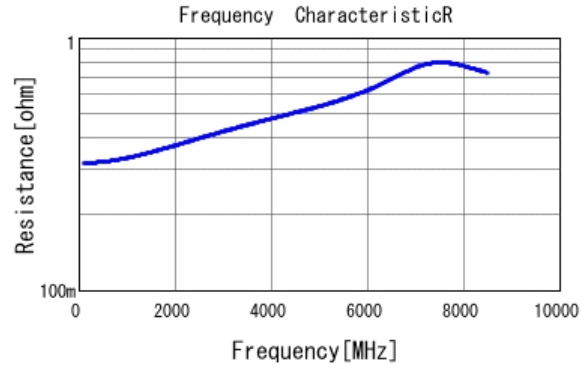
■ GCM1555C1H2R0BA16 R DCOV, 25degC
