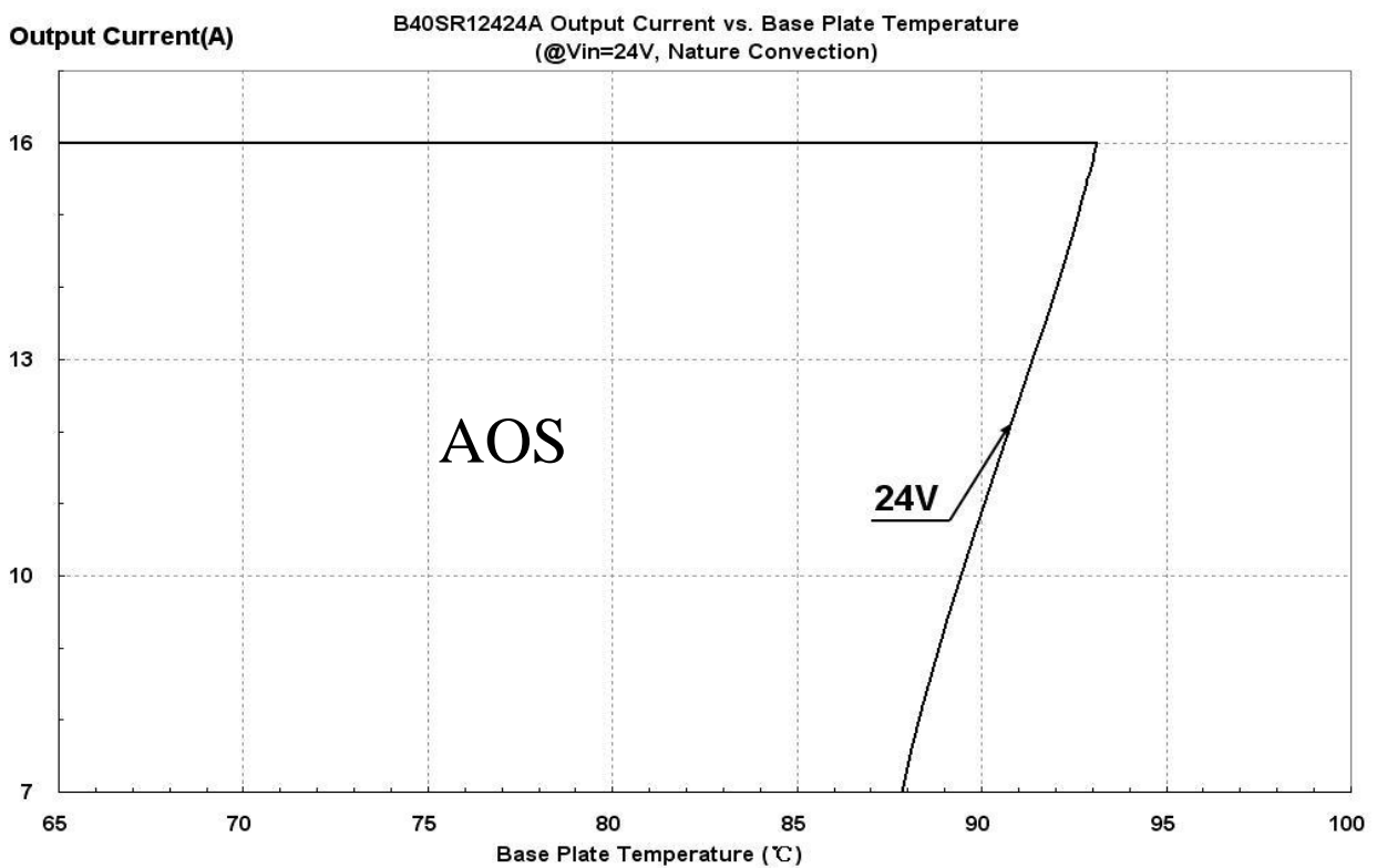
Figure 18: Output Current vs. Base Plate temperature
