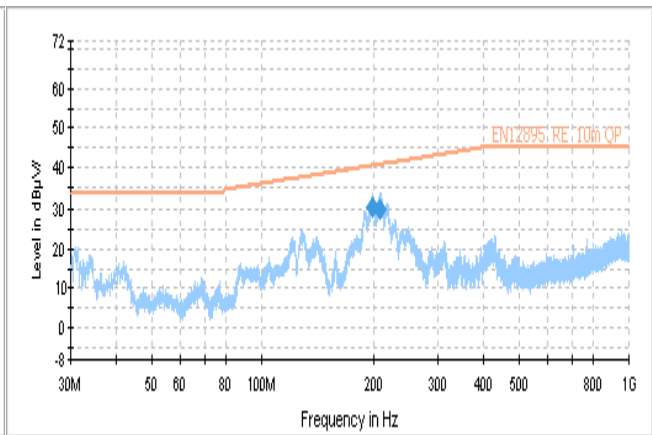
Figure 16: test result(Horizontal)
