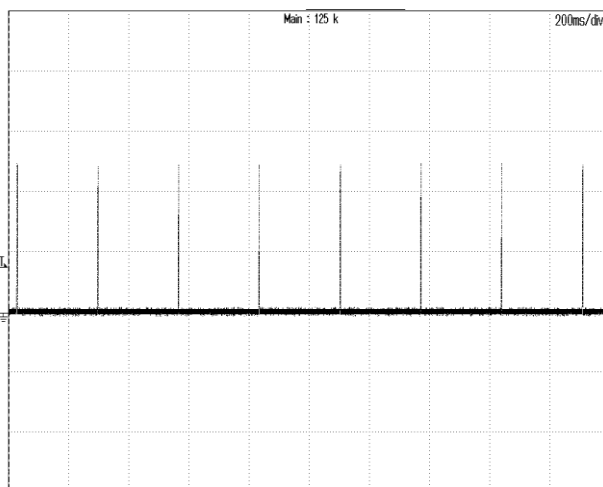
Figure 11: Output short current @ V_{in}=48V CH1:io, 20A/div, 200ms/div
