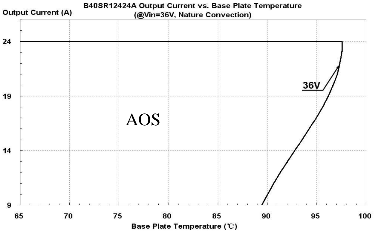
Figure 19: Output Current vs. Base Table temperature @ Vin=36V
