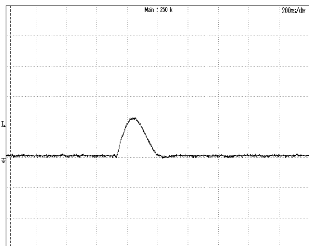
Figure 12: Inrush current @ V_{in}=48V CH1:lin, 2A/div, 200ns/div Max current 2.7A, I_2t=1.24E-7 A^2S
