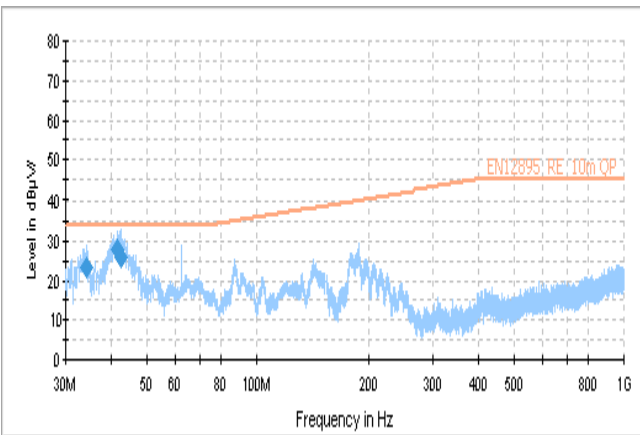
Figure 15: test result(Vertical)
