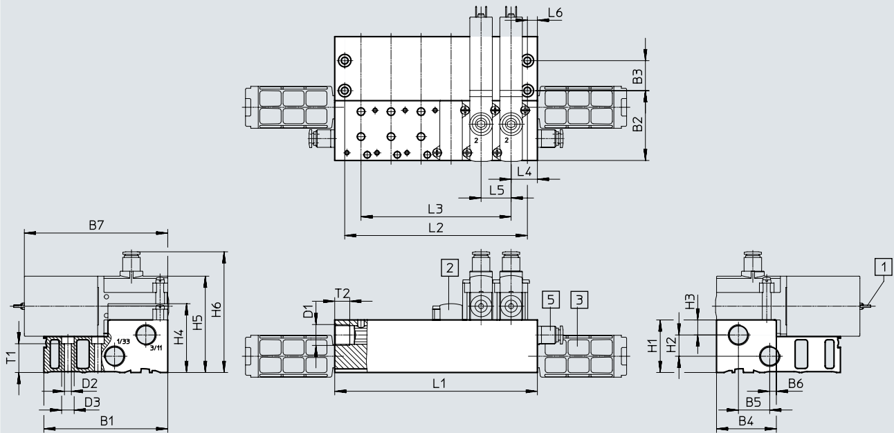
[1] Plug vanes [2] Cover plate [3] Silencer [5] Push-in fitting
