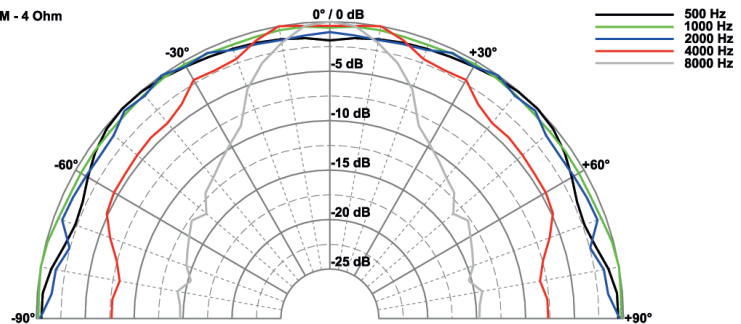
SL 87 WPM - 4 Ohm
