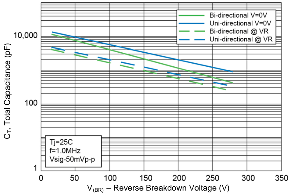
FIGURE 4 Typical Junction Capacitance
