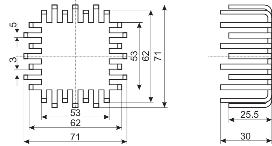
105 71x71x30 mm
