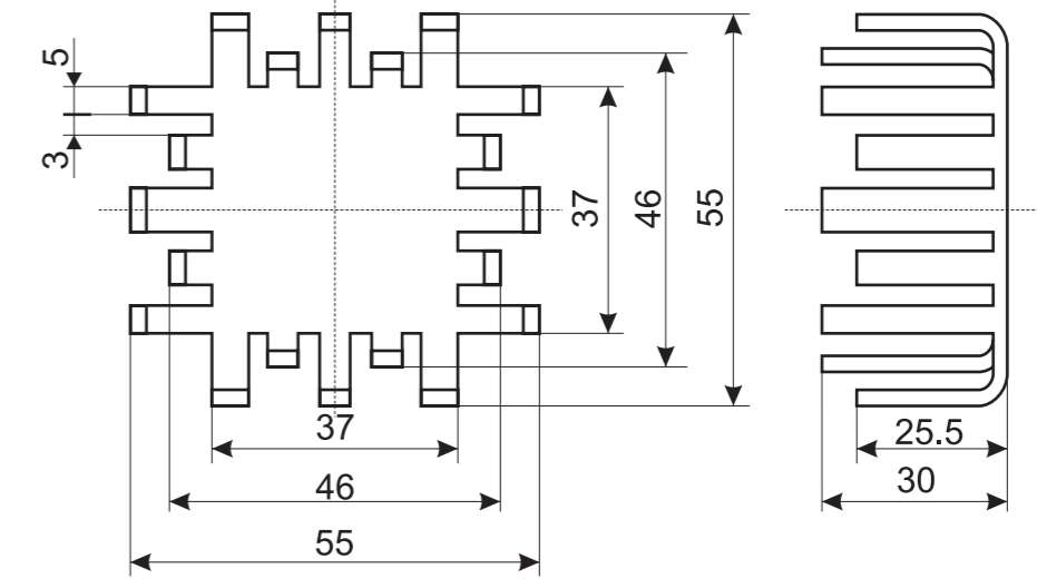
103 55x55x30 mm
