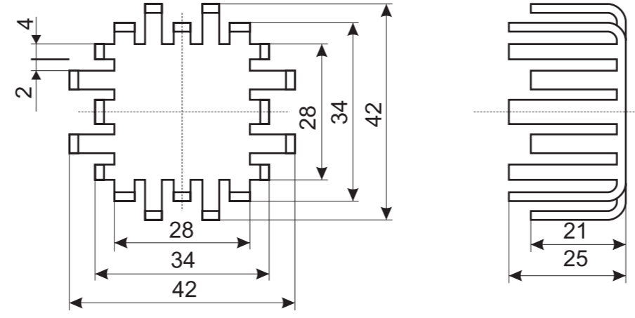
102 42x42x25 mm
