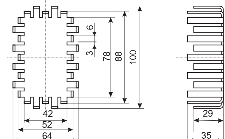
203 64x100x35 mm
