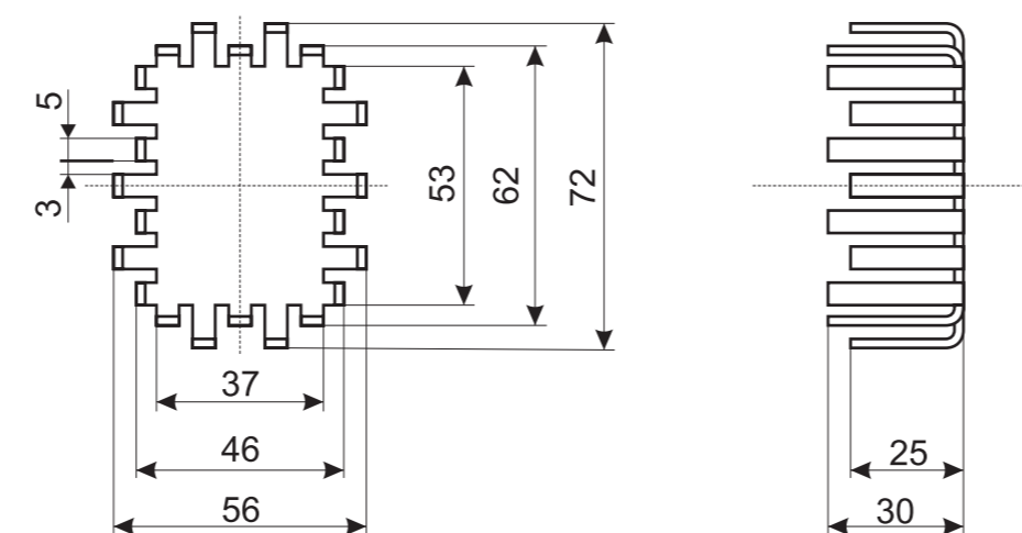
202 56x72x30 mm
