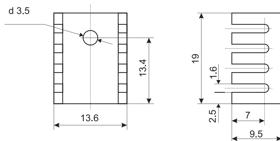
718 19x13.6x9.5 mm
