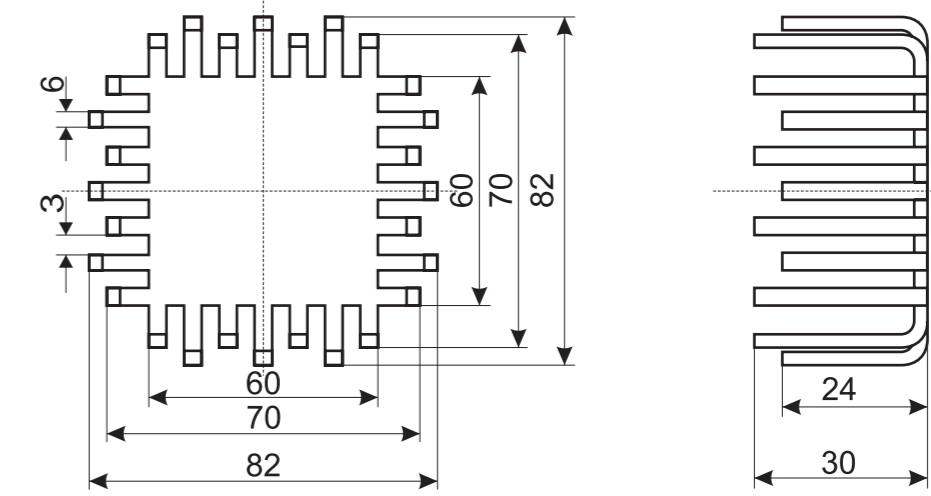
106 82x82x30 mm
