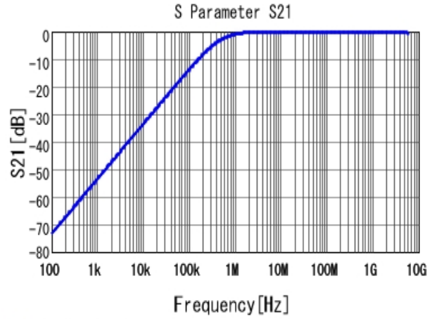
■ GCD188R71H332KA01 S21 DCOV, 25degC
