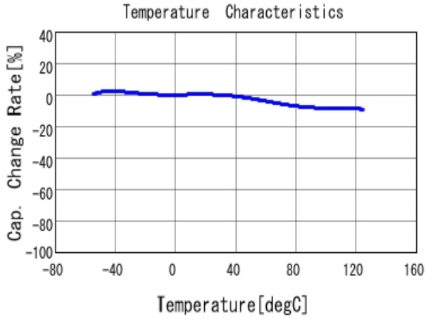
■ GCD188R71H332KA01 C-Temp. capchange, DCO. 0V, AC1.0V rm
