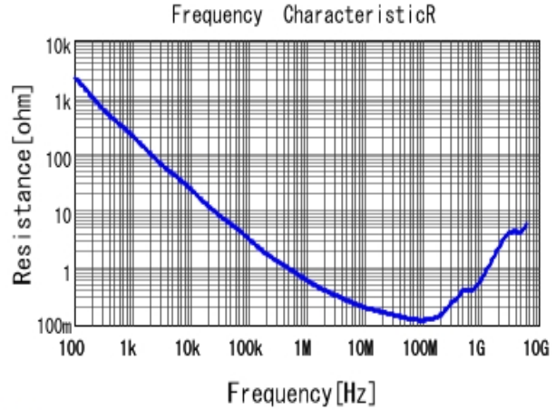
■ GCD188R71H332KA01 R DCOV, 25degC
