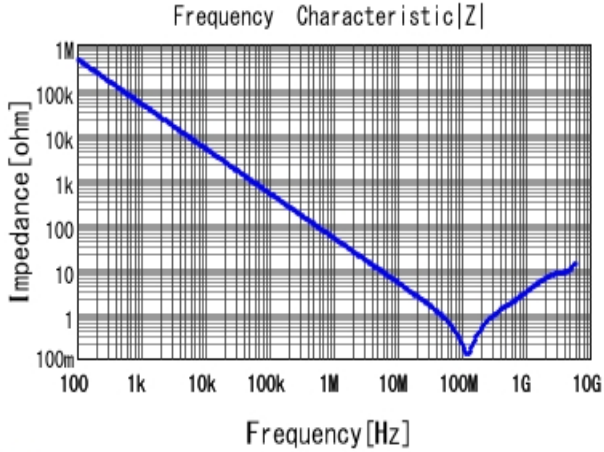
■ GCD188R71H332KA01 |Z| DCOV, 25degC
