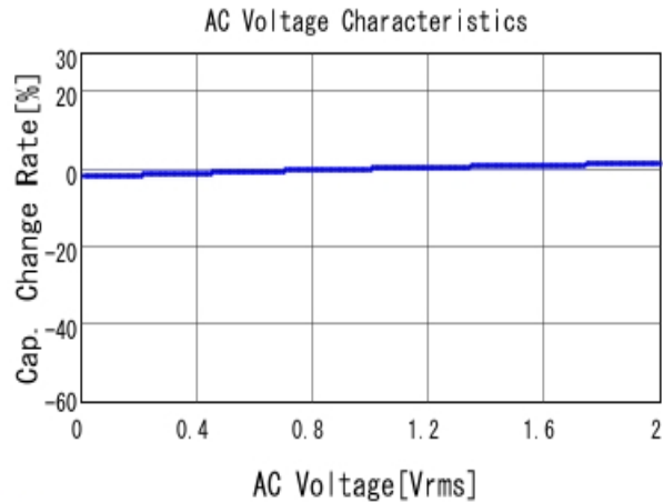
■ GCD188R71H332KA01 C-AC Voltage capchange, DCOV, 25.0d
