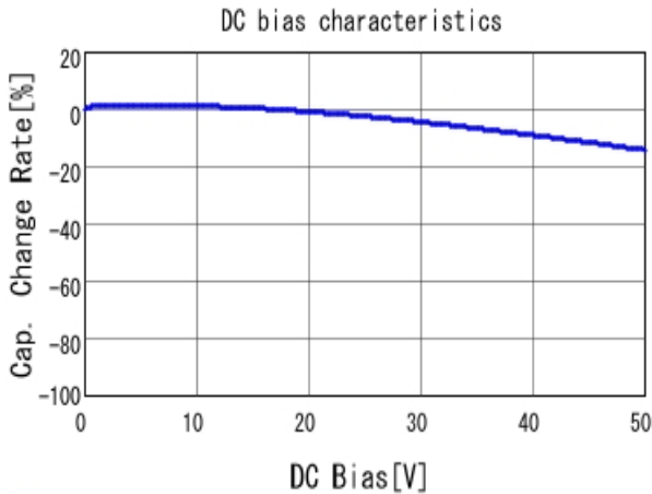
■ GCD188R71H332KA01 C-DC bias capchange, 25.0degC, AC1.
