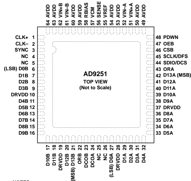
Figure 5. Pin Configuration
