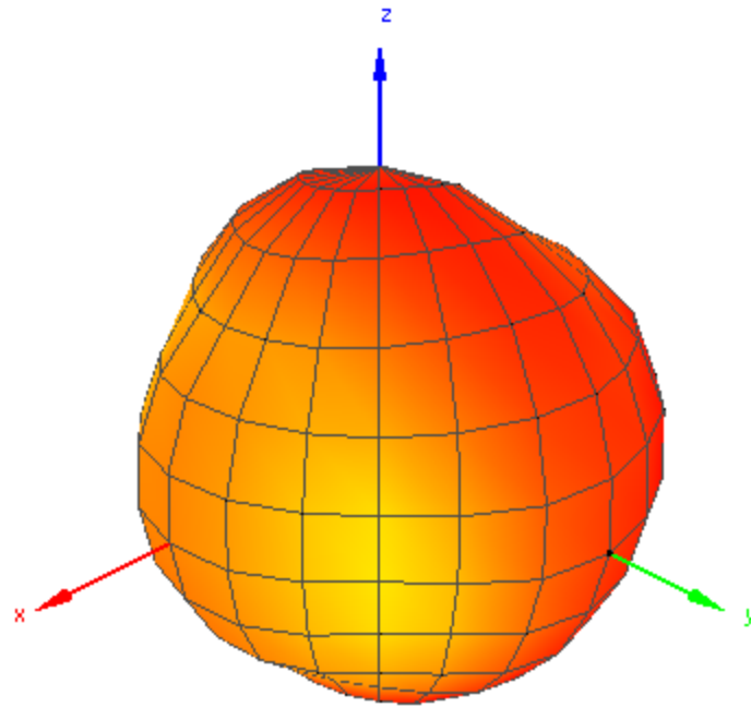
Figure 11. Radiation Pattern at 1575 MHz of FXUB63 Antenna.
