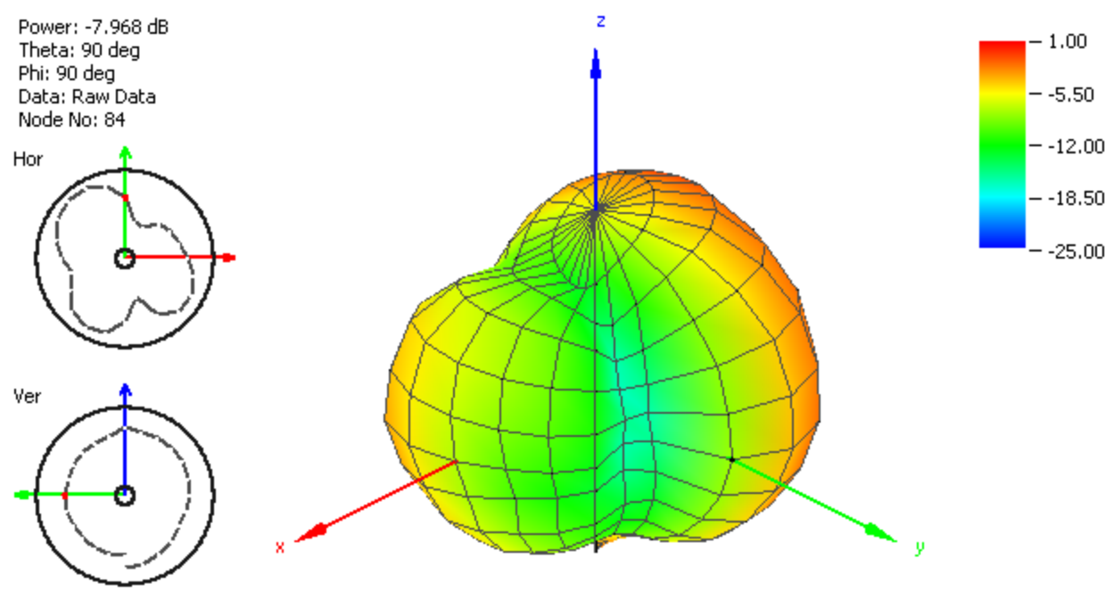
Figure 8. Radiation Pattern at 850 MHz of FXUB63 Antenna.
