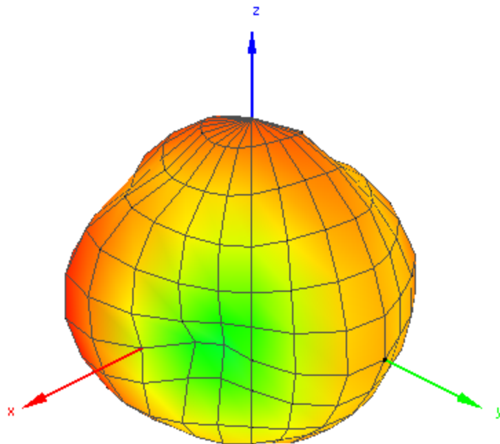
Figure 12. Radiation Pattern at 1750 MHz of FXUB63 Antenna.
