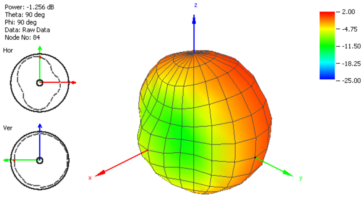
Figure 7. Radiation Pattern at 750 MHz of FXUB63 Antenna.
