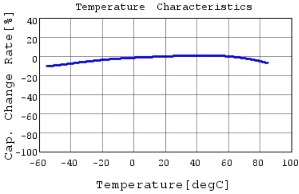
GRM319R61C106KE15 C-Temp. capchange, DC0.0V,
