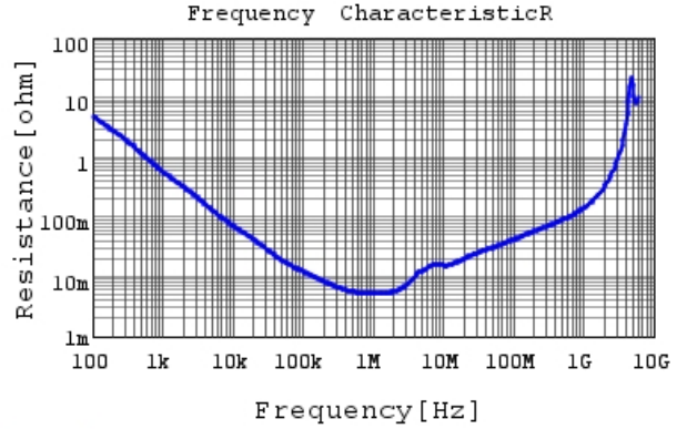
GRM319R61C106KE15 R DCOV,25degC
