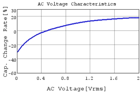
GRM319R61C106KE15 C-AC Voltage capchange, Dc
