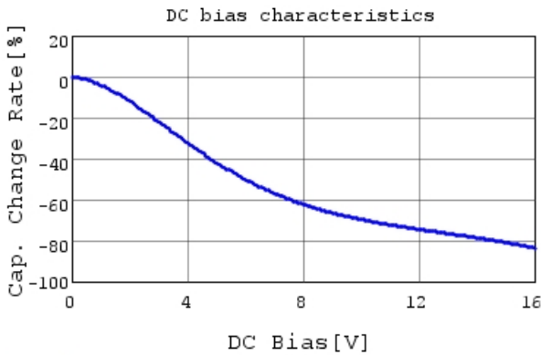
GRM319R61C106KE15 C-DC bias capchange, 25.0c
