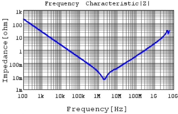
GRM319R61C106KE15 |Z| DCOV,25degC
