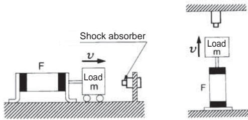
RJ0806H Absorbed Energy
