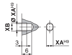
Detailed figure of section XX
