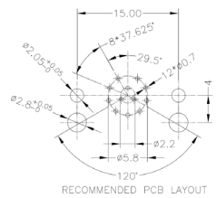
12 Contact PCB Layout
