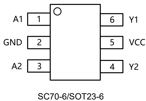
Figure1. Top View
