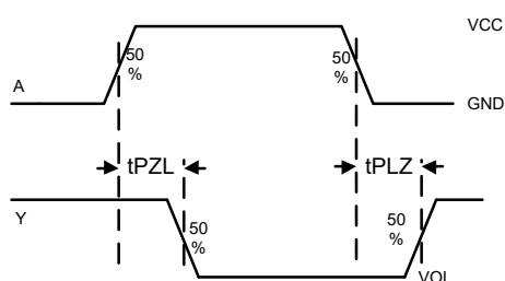
Figure 3. Switching Waveform
