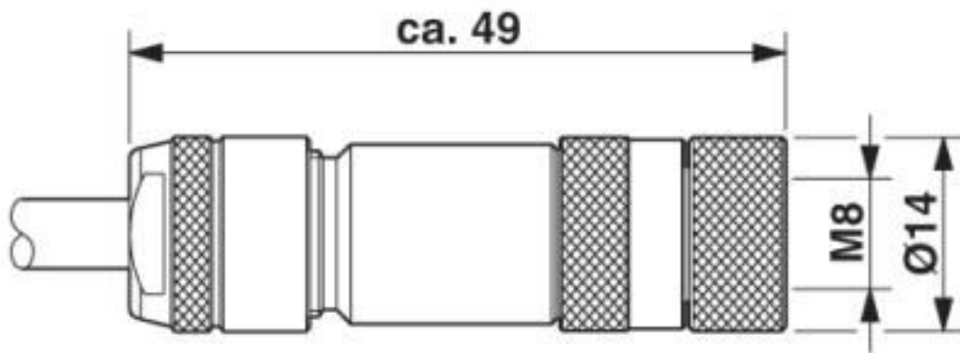
Dimensional drawing
