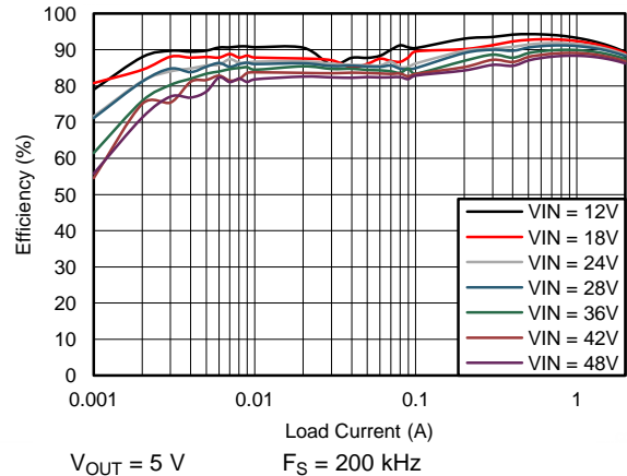
Figure 60. Efficiency
