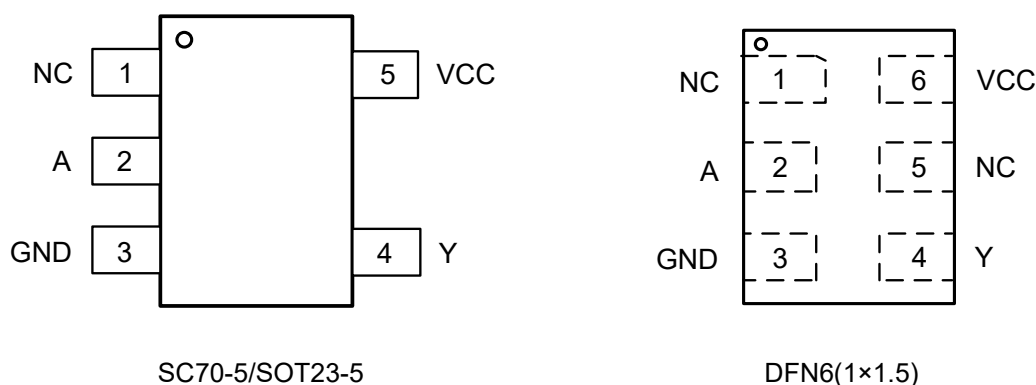
Figure1. Top View
