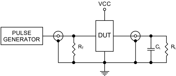
R_T = 50\Omega \text{ (typ)} Figure4. Test Circuit
