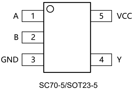
Figure1. Top View
