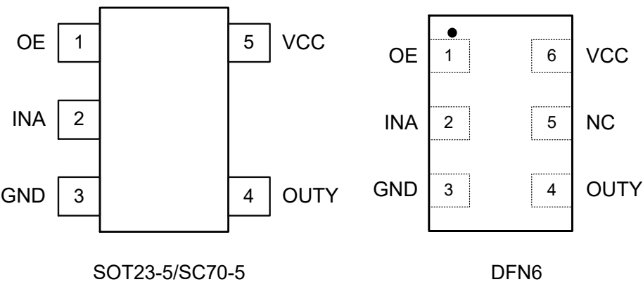
Figure1. Top View
