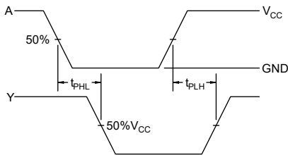
Figure 3. Switching Waveforms
