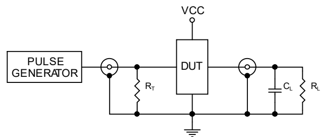
Figure4. Test Circuit
