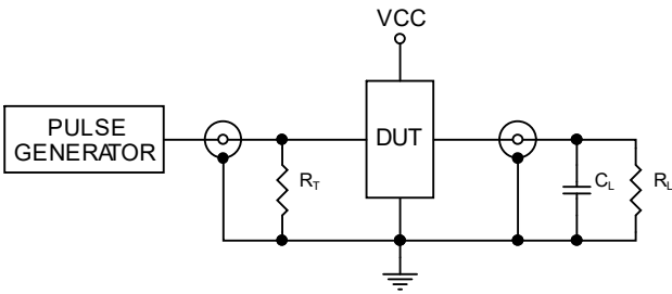
Figure4. Test Circuit
