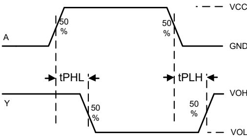
Figure 3. Switching Waveform
