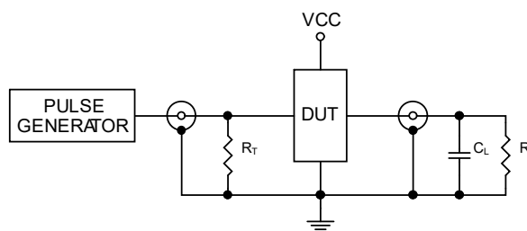
Figure4. Test Circuit
