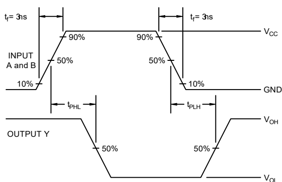
Figure3. Switching Waveform
