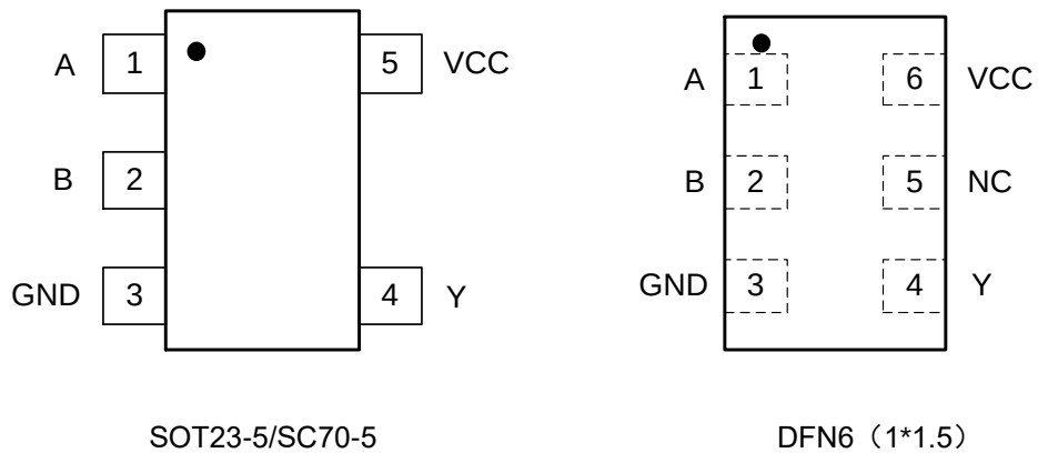
Figure1. Top View
