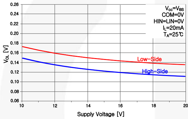
Figure 25. Low-Level Output Voltage vs. Supply Voltage
