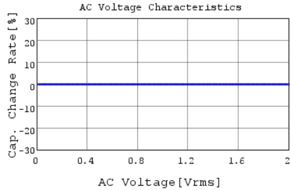
GJM1555C1H2R0CB01 C-AC Voltage capchange, Dc
