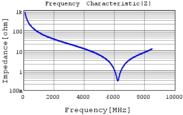
GJM1555C1H2R0CB01 |Z| DCOV, 25degC
