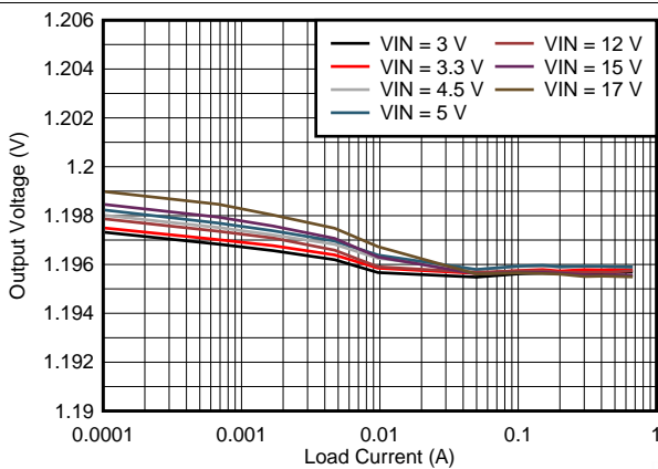
Figure 30. Line and Load Regulation V_{OUT} = 1.2V
