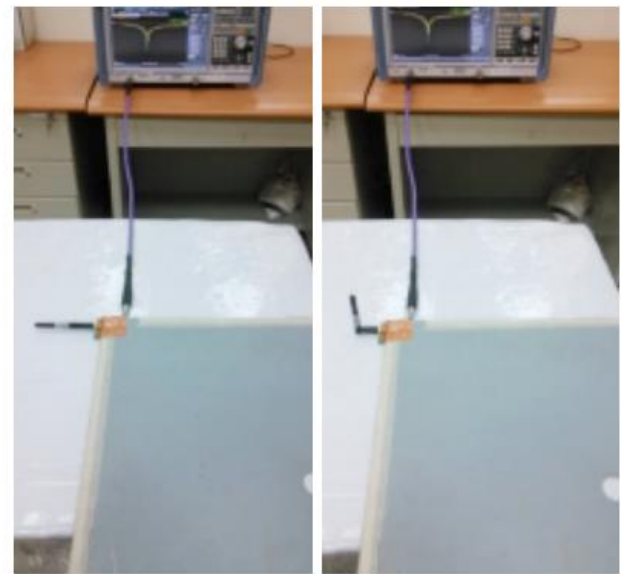
Antenna straight
