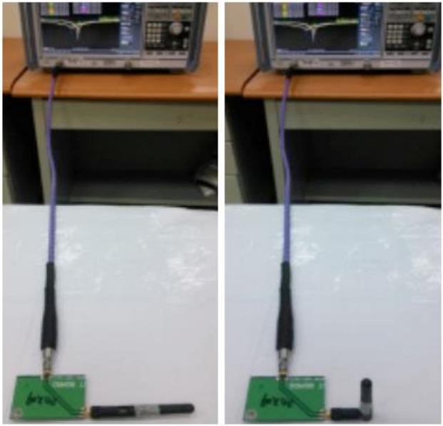
Antenna straight
