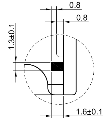
POLARITY PROTECTION DEVICE DETAIL "A" S=3
