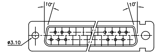
VIEW OF MATING FACE
