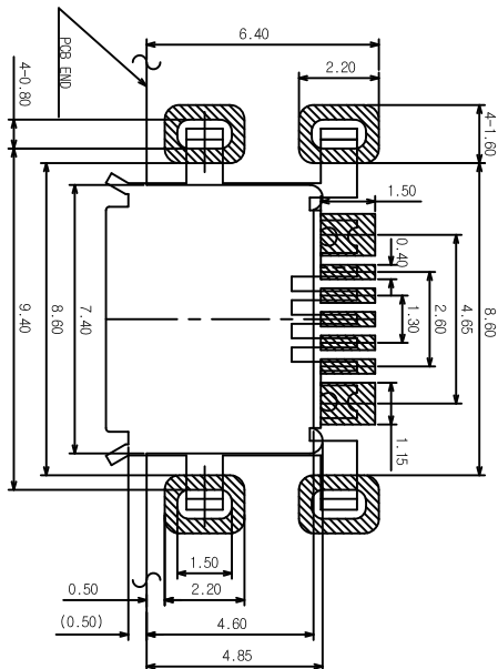
USB-IF REVERSE type Pattern USB-IF Recommended REVERSE type Pattern (Tolerance : ±0.05)
