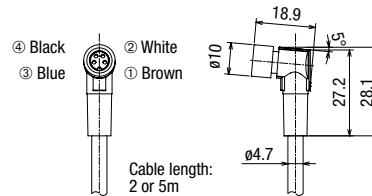
Right-angle (SA9Z-CM8K-4L□)
