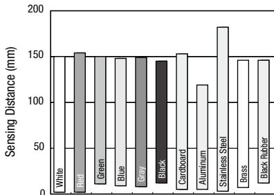
Comparison of sensing distance when set to detect white matte paper (100 × 100 mm) at 150 mm
