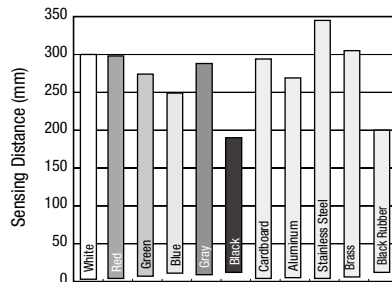
Comparison of sensing distance when set to detect white matte paper (100 × 100 mm) at 300 mm
