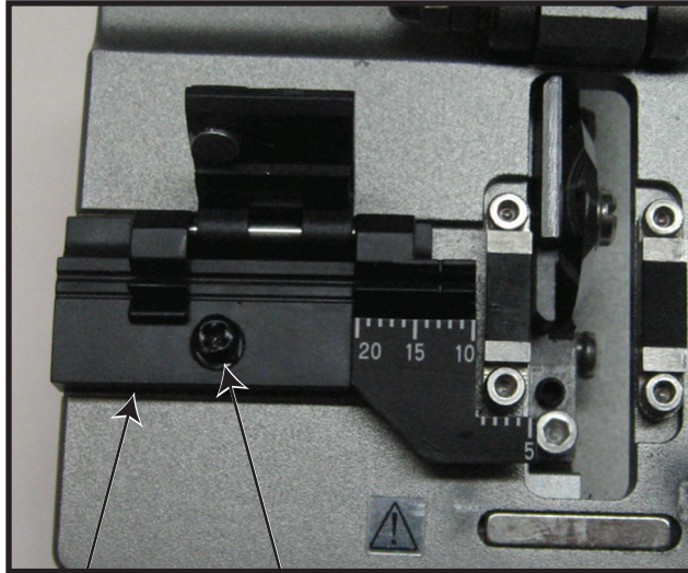
Fixed Clamp Mounting Screw
