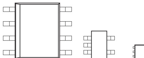
Package Footprint Comparison (to Scale)
