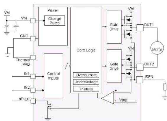
Figure 1. NSD7312 Block Diagram
