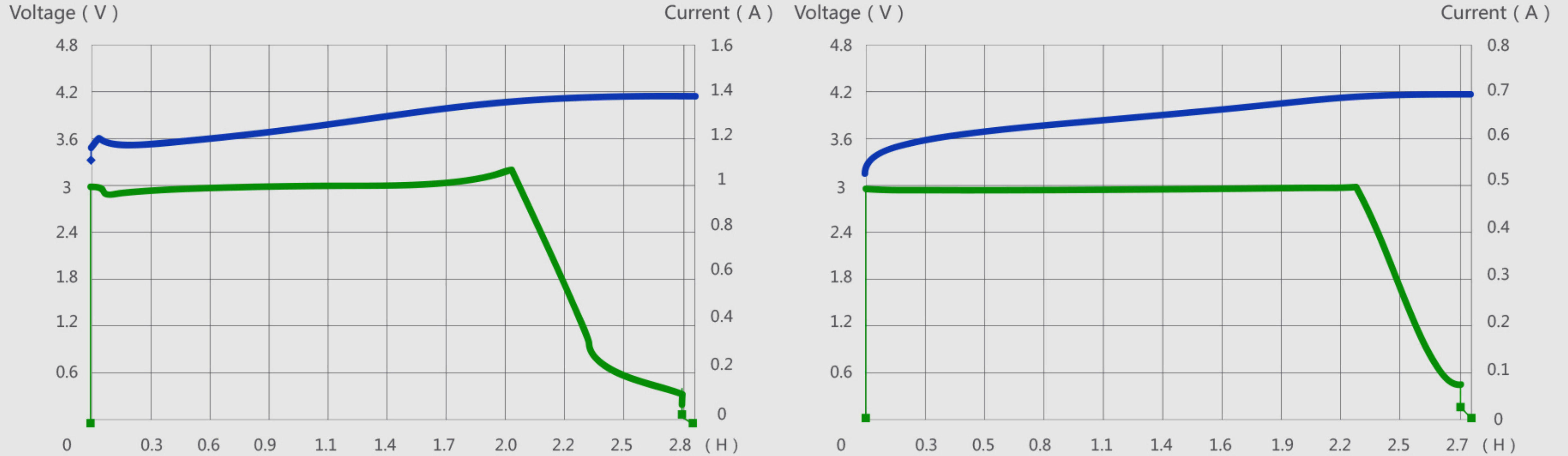
Li-ion: XTVTC4/2200mAh-1.0A
