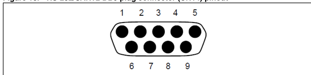
Figure 18. RS-232/UART2 DB9 plug connector (CN14) pinout
