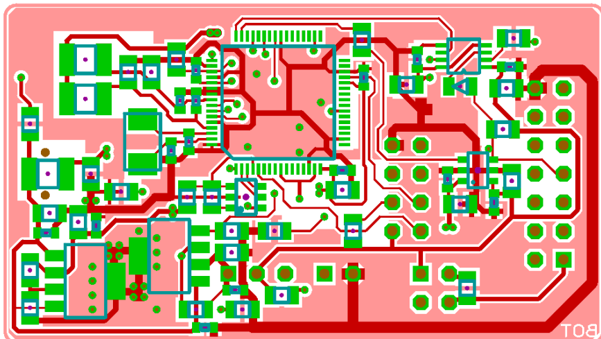
Figure 9. HiCom Communication Board Layout - Bottom Layer
