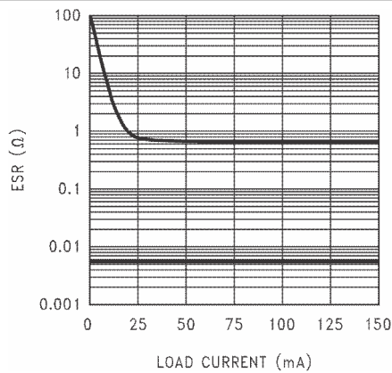
Figure 6-19. 4.7- \mu\text{F} Stable ESR Range for Output Voltage \leq 2.3 \text{ V}
