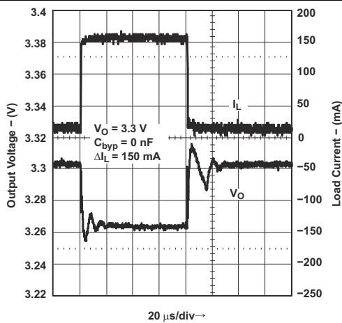
Figure 8-6. Load Transient Response
