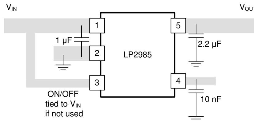
Figure 10-1. Layout Diagram
