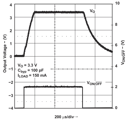
Figure 8-12. Turn-On Time
