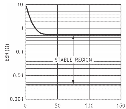
Figure 6-18. 2.2- \mu\text{F} Stable ESR Range for Output Voltage \leq 2.3 \text{ V}
