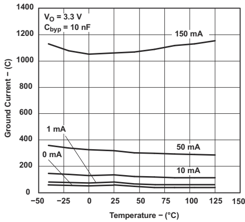
Figure 6-17. Ground-Pin Current vs Temperature
