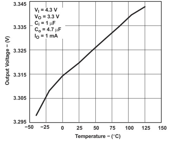
Figure 6-2. Output Voltage vs Temperature
