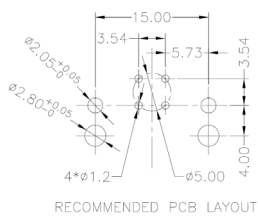
4 Contact PCB Layout
