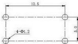
Mounting
