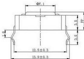
Outline Drawing
