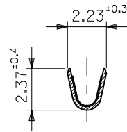
SECT. B-B
