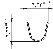
SECT. A-A
