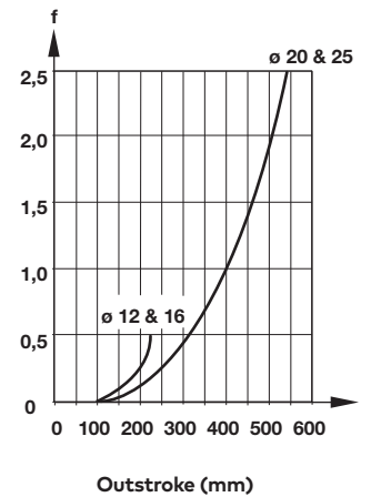
Deflection (mm)
