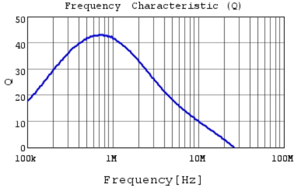
1277AS-H-4R7M Q
