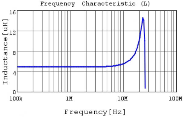
1277AS-H-4R7M L
