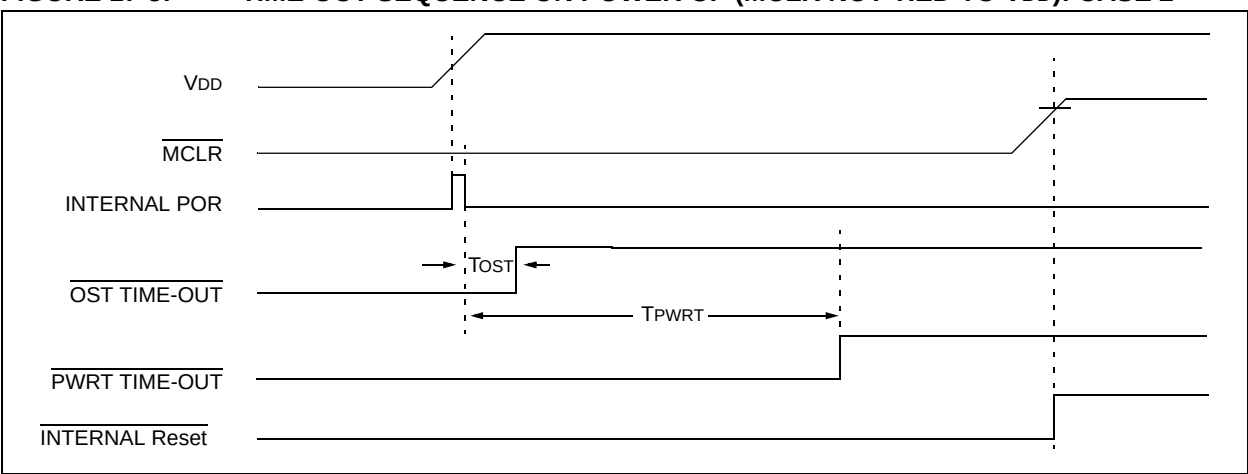
FIGURE 17-5: TIME-OUT SEQUENCE ON POWER-UP ( \overline{\text{MCLR}} NOT TIED TO V_{DD} ): CASE 2
