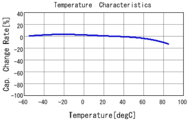
GRT188R61A106KE13 C-Temp. capchange, DCO. 0V, ACO. 5Vrm
