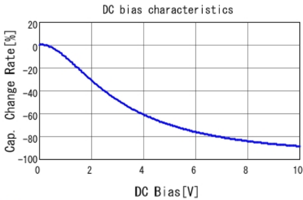
GRT188R61A106KE13 C-DC bias capchange, 25.0degC, AC0.
