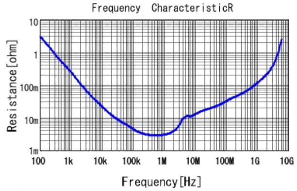
GRT188R61A106KE13 R DCOV, 25degC
