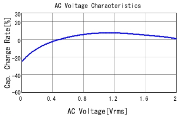
GRT188R61A106KE13 C-AC Voltage capchange, DCOV, 25.0d
