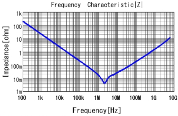
GRT188R61A106KE13 |Z| DCOV, 25degC
