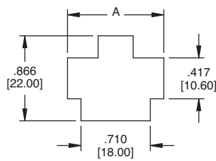
Recommended Panel Cut-Out For 1.50mm Panel Thickness
